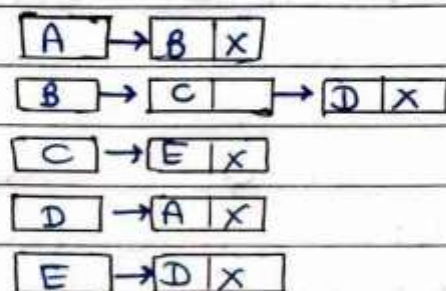
Fig: Adjacency list
